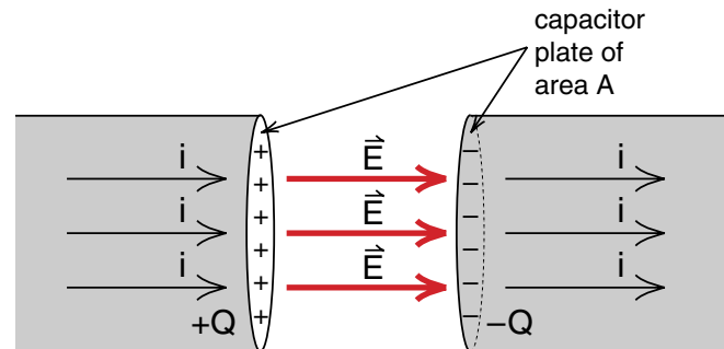
Figure 6 An electric field \vec{E} exists between the plates.
