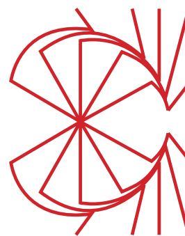
Figure 35c Field of a charge that stopped. Assume that the charge stopped t seconds ago. Inside a circle of radius ct , we have the field of a stationary charge. Outside, where there is no information that the charge has stopped, we still have the field of a moving charge. The kink that connects the two fields is the electromagnetic radiation.
